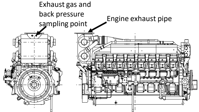
Fig.1 S16R-PTAW Engine
