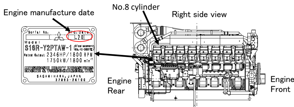
Fig.4 Name Plate Position (S16R-PTAW)
