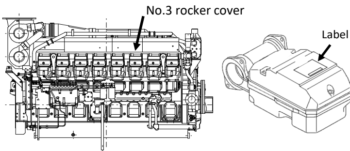
Fig.2 Label Position (S16R-PTAW)
