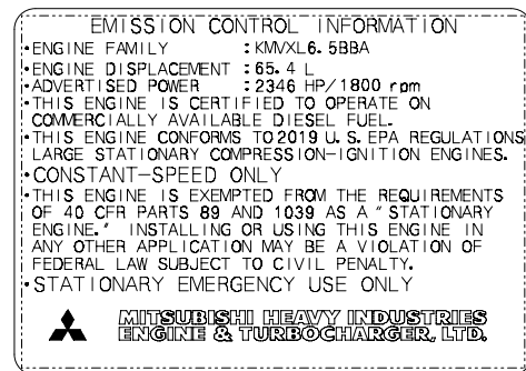
Fig.3 Emission Control Information Label
