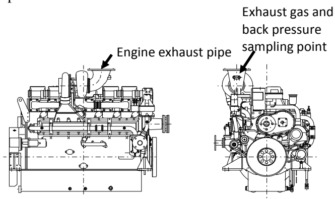
Fig.1 S6R-PTAW Engine
