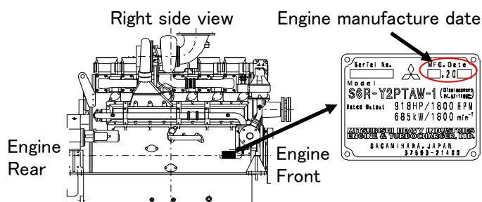
Fig.4 Name Plate Position (S6R-PTAW)
